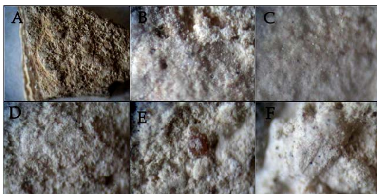
Fig. 12. Optical photomicrographs of different rendering layers from both temples under stereomicroscope:
