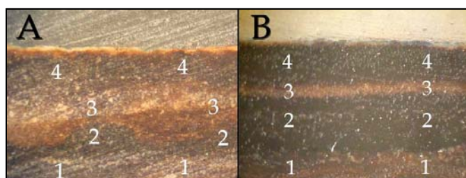
Fig. 11. Optical photomacrography of polished cross sections samples:
