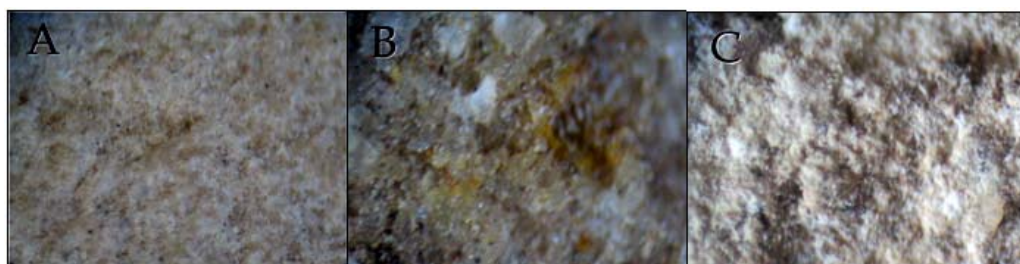
Fig. 6. Optical photomacrography of stone and mortar samples from the temple of Seti I under stereomicroscope: A -Limestone sample shows homogeneous fine-grained structure (70X); B -Sandstone sample shows particles of quartz differ in their size. In their shape, they are angular and sub-rounded. Some particles are coated with red/yellow color (70X); C - Mortar sample shows the presence of fine quartz particles (70X).
